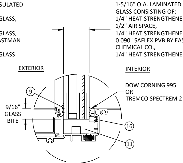
GLAZING DETAIL F (WET GLAZED)
