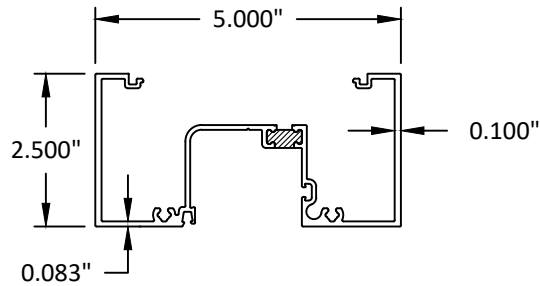
1 HEAD/JAMB/VERTICAL
