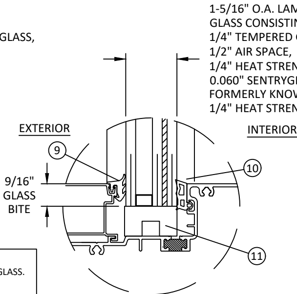
GLAZING DETAIL H (DRY GLAZED)
