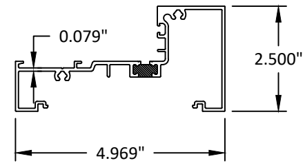
3 SILL
