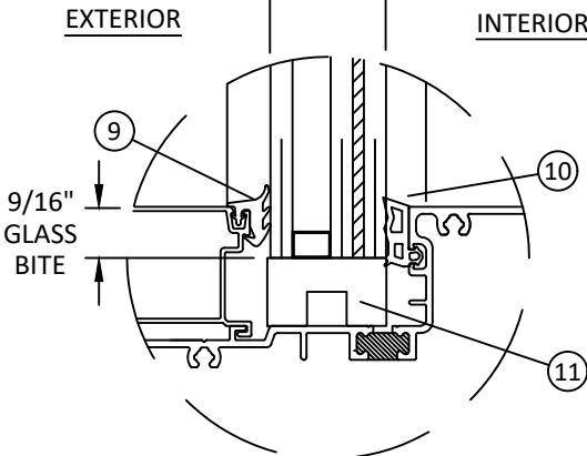
GLAZING DETAIL D (DRY GLAZED)
