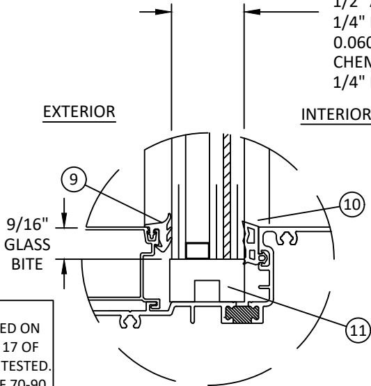
GLAZING DETAIL B (DRY GLAZED)
