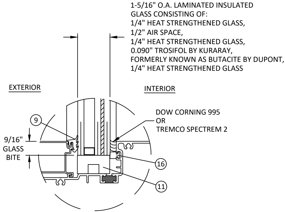
GLAZING DETAIL G (WET GLAZED)
