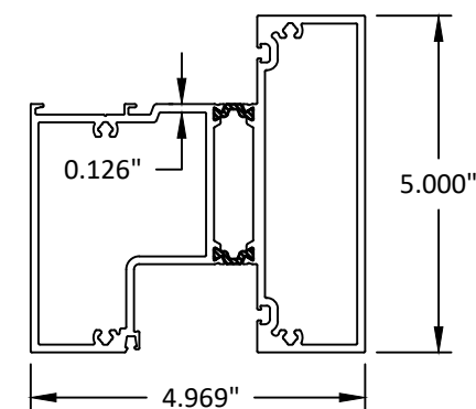
22 5" HORIZONTAL
