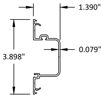
7 HEAVY DUTY VERTICAL
