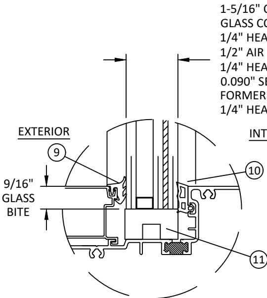
GLAZING DETAIL A (DRY GLAZED)
