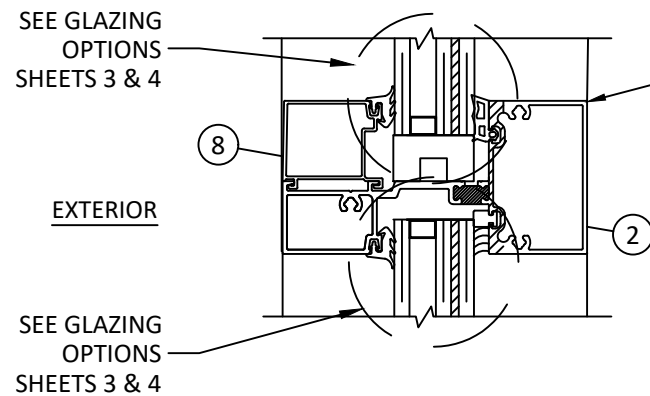
B 10 VERTICAL SECTION HORIZONTAL MEMBER
