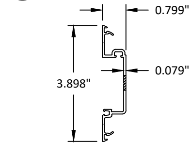
6 SHALLOW POCKET FILLER
