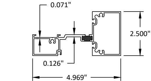
2 HORIZONTAL
