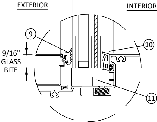
GLAZING DETAIL C (DRY GLAZED)
